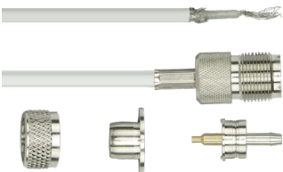
Coaxial Extension - PL259 Connector (5M)
